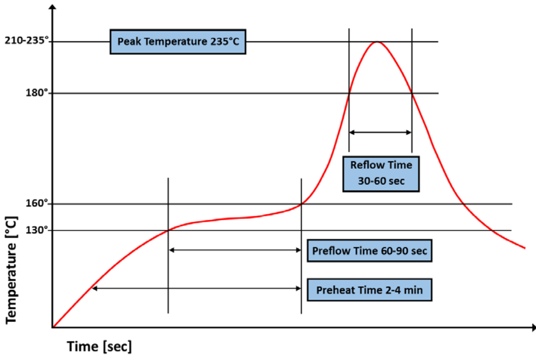
Figure 1 – Low Temperature Solder Reflow Thermal Profile
