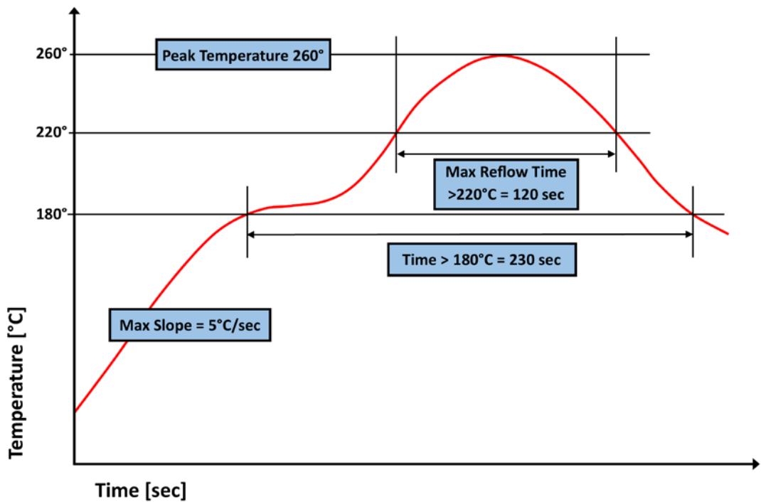
Figure 2 – High Temperature Solder Reflow Thermal Profile
